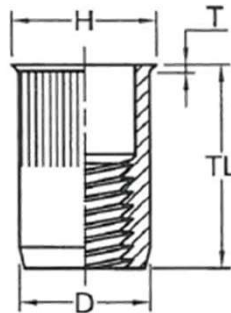
Countersunk
