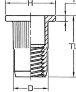
Large Flange
