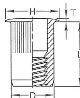
Large Flange
